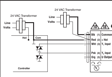
Triac Sink with Separate Transformer
