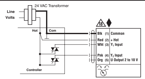
Triac Source
