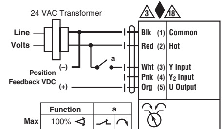
Triac Sink
