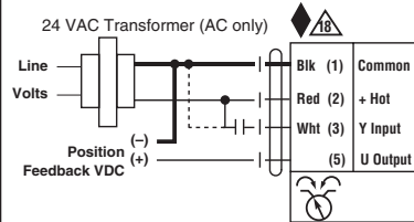
Triac Sink with Separate Transformer
