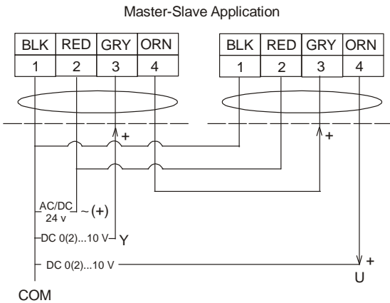
Figure 9: Control Wiring
