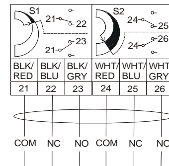
Figure 11: Auxiliary Switch Wiring Diagram
