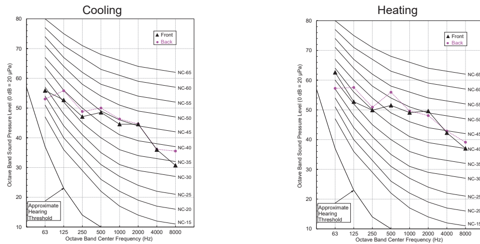
Figure 15: Sound Pressure Levels for LSU240HEV2, LSU240HFV3 Outdoor Units.
