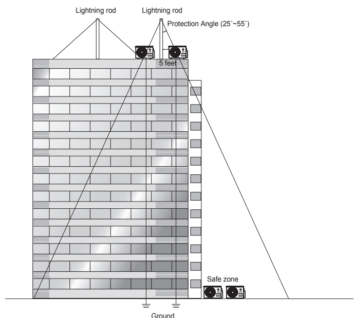
Figure 33: Lightning Protection Diagram.
